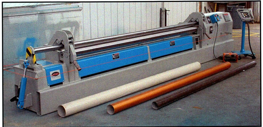
KRR-3.5-120 rigidified top roll initial pinch rolling gutter down spouts
