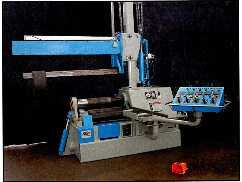
403-8(6)-2 with infeed table and overhead/ejector rolling manhole cover risers
